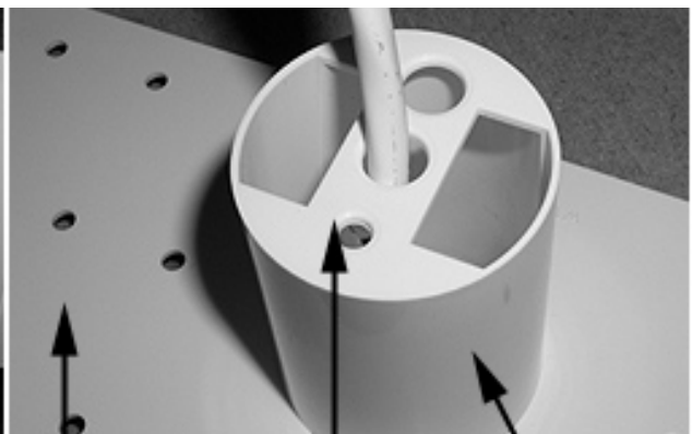
Bridge Wire Inlet Holes Wire Cavity
