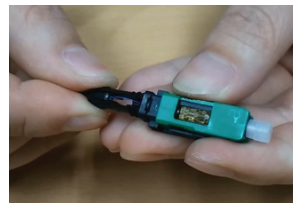
Insert the fiber into the connector body until the strand meets resistance and bows slightly
