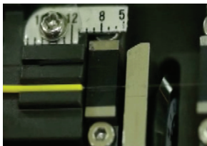
Cleave your fiber strand to 10mm from the 250μm measurement mark
