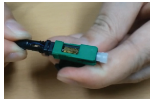
To remove or re-terminate the connector, simply unscrew the boot and replace the jig
