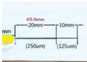
Measure from the end of the jacket and make a mark between the 250μm and 125μm section
