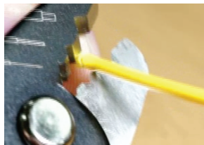
Strip outer jacket about 50mm to reveal 900-micron fibers
