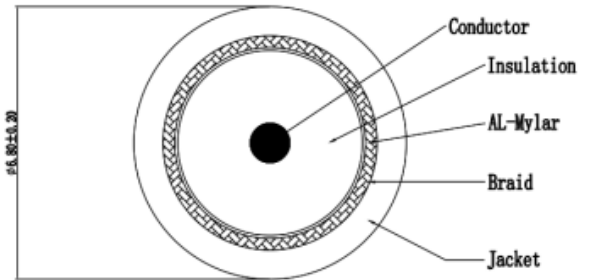
CABLE SECTION
